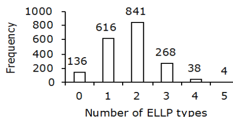
Fig 3. ELLP diversity
