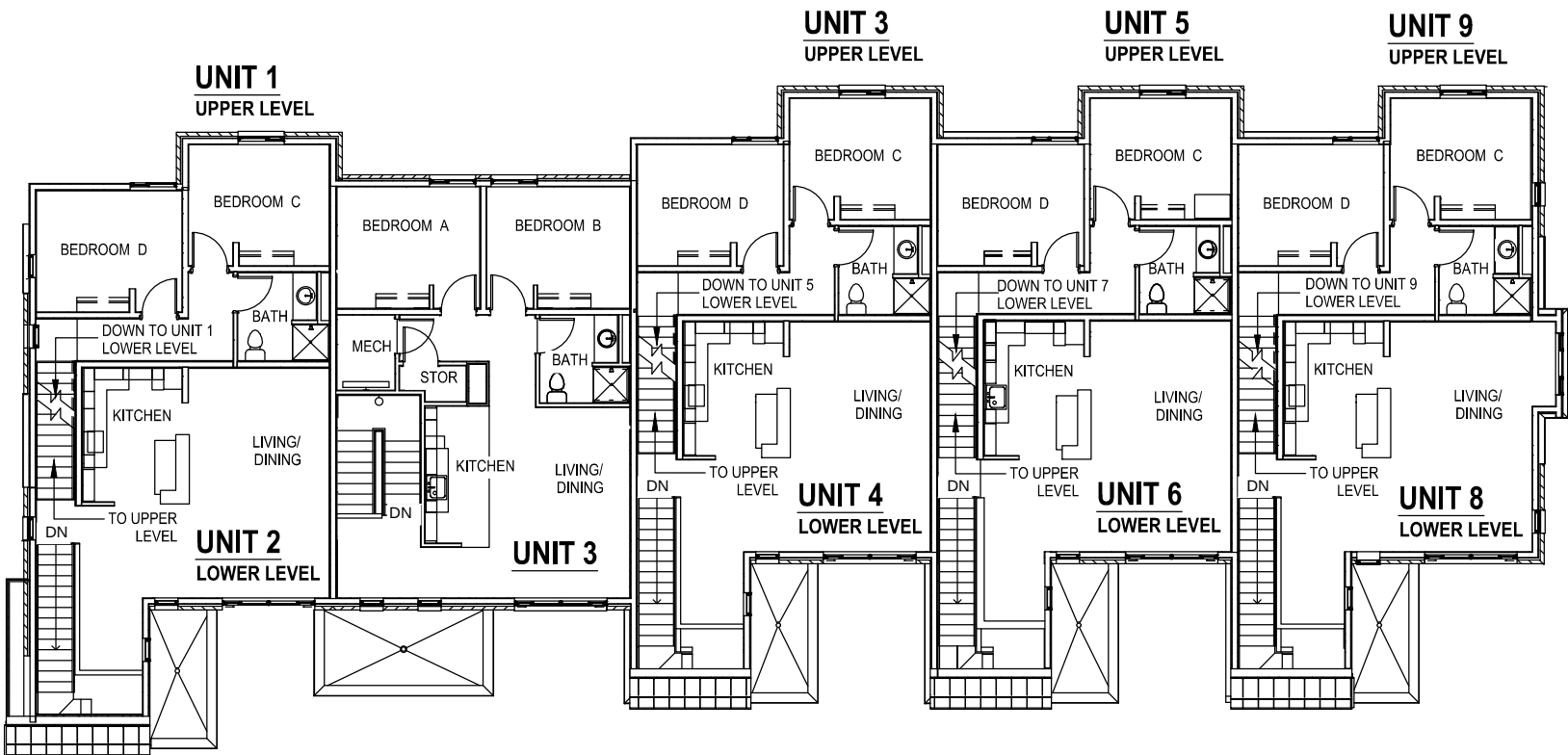
SECOND FLOOR PLAN - BUILDINGS "F", "G" and "I"
