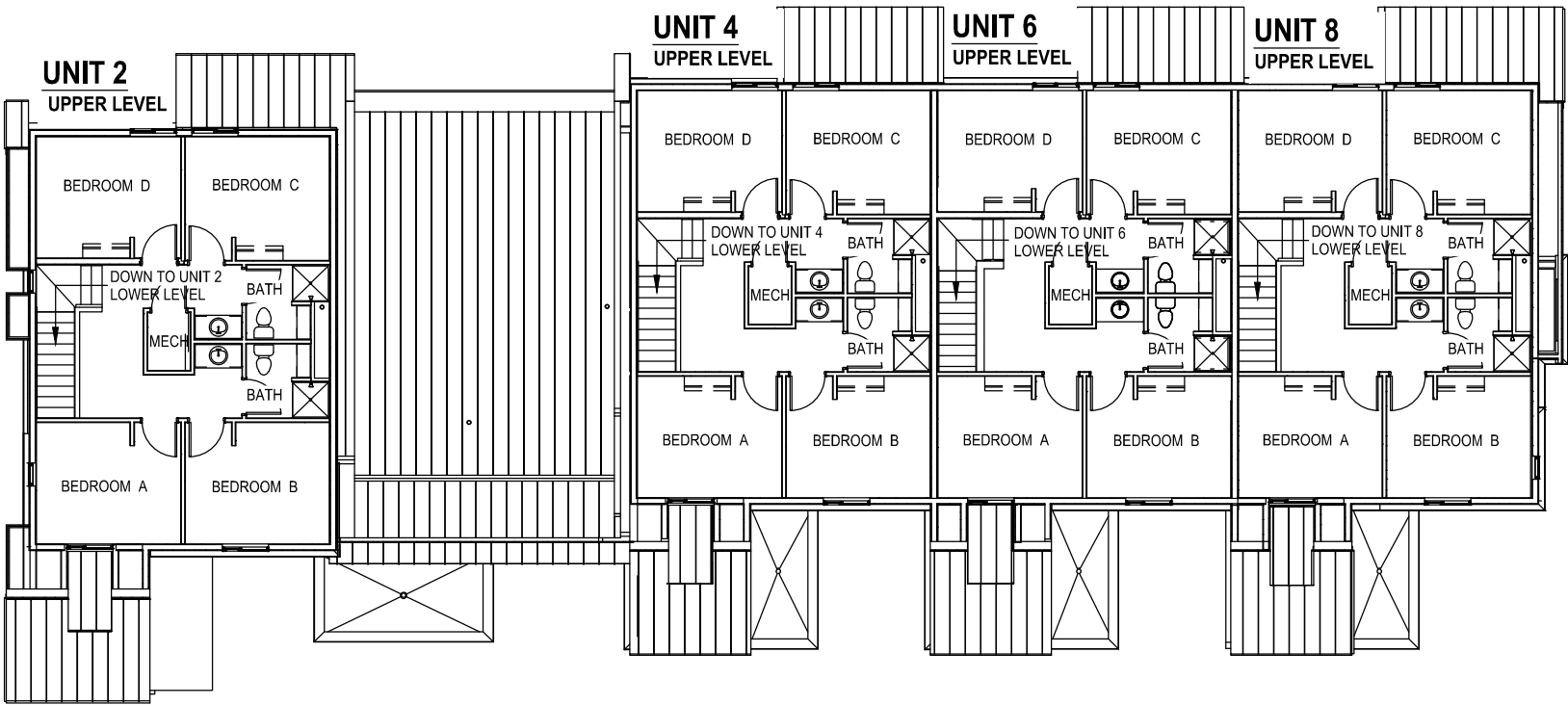
THIRD FLOOR PLAN - BUILDINGS "F", "G" and "I"
