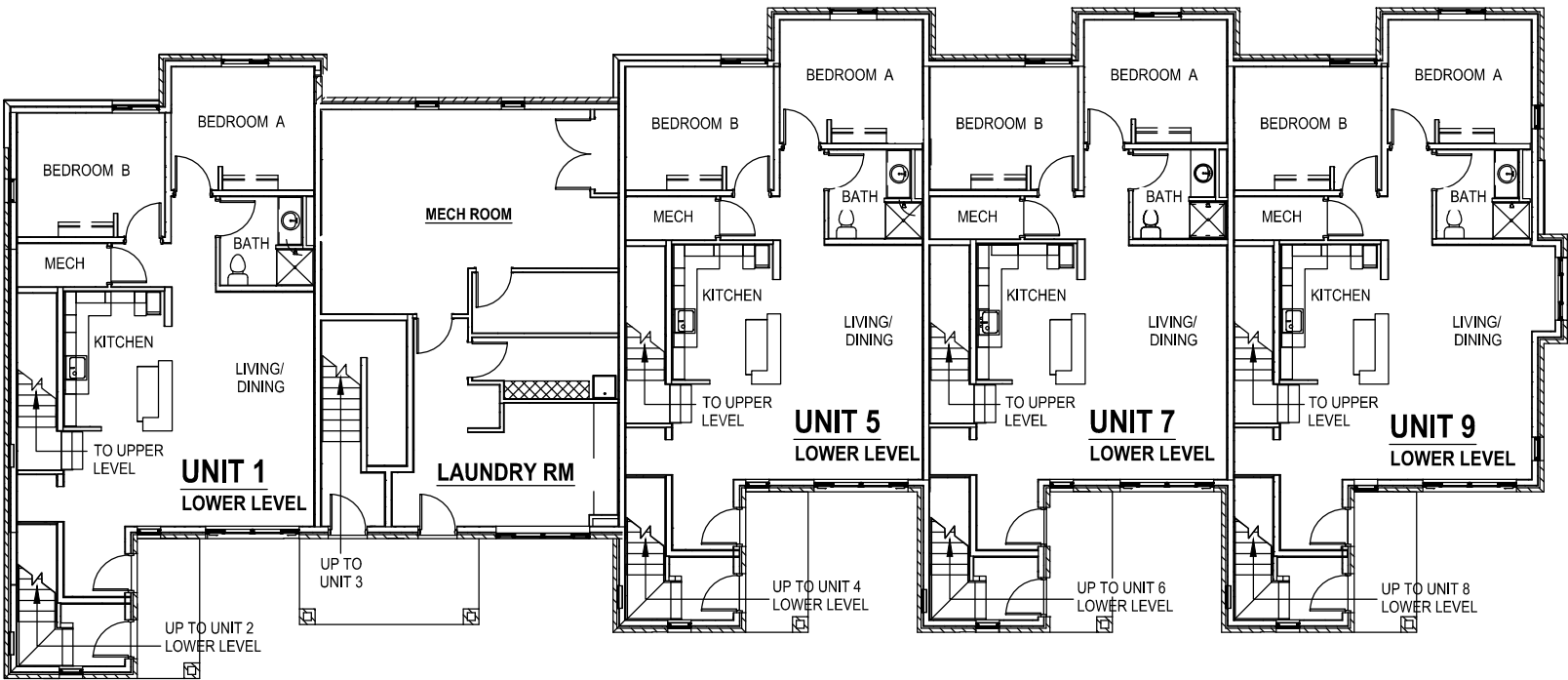
FIRST FLOOR PLAN - BUILDINGS "F", "G" and "I"
