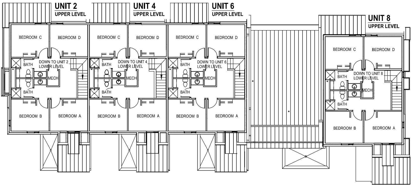
THIRD FLOOR PLAN - BUILDINGS "H", "J", "K" and "L"
