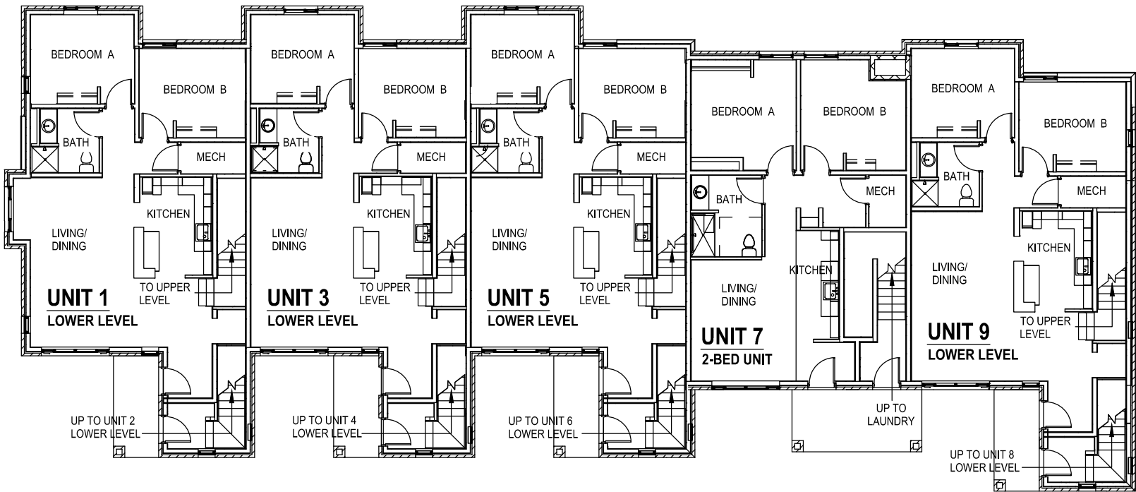
FIRST FLOOR PLAN - BUILDINGS "H", "J", "K" and "L"
